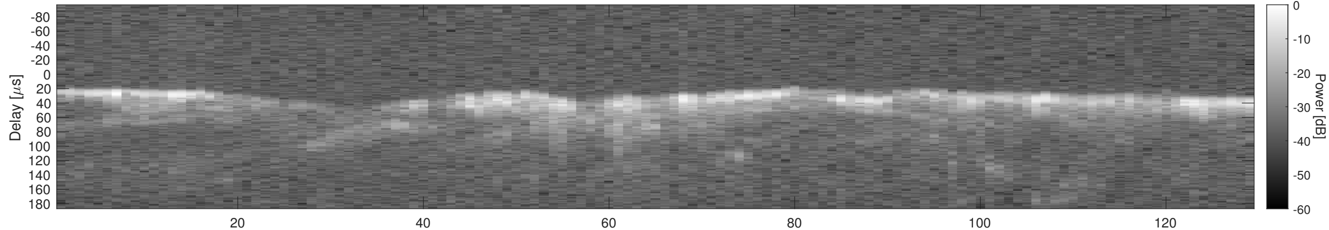
Orbit 4931, Window, Channel 2, Chapman
