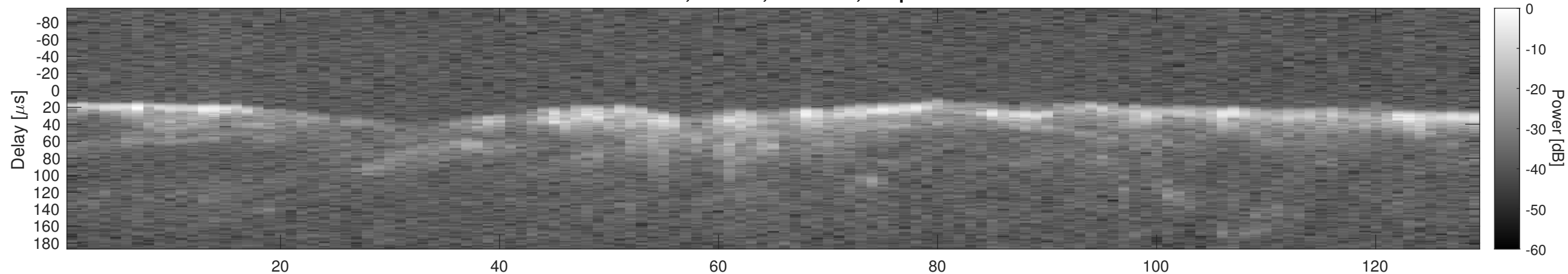
Orbit 4931, Window, Channel 2, Optimized
