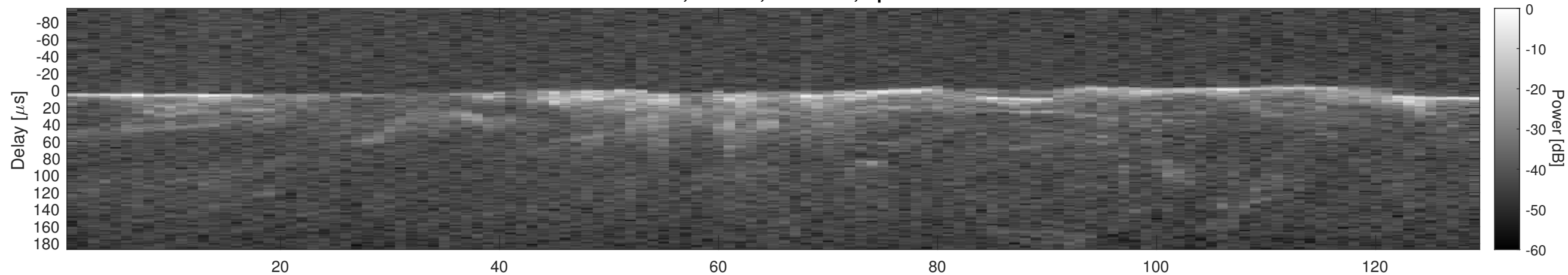
Orbit 4931, Cluttergram
