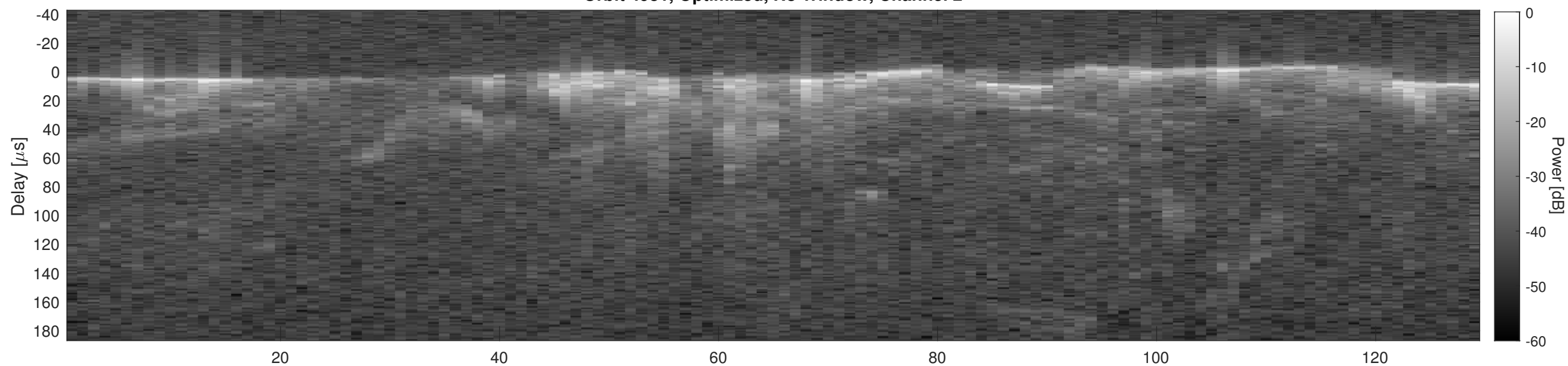
Orbit 4931, Cluttergram
