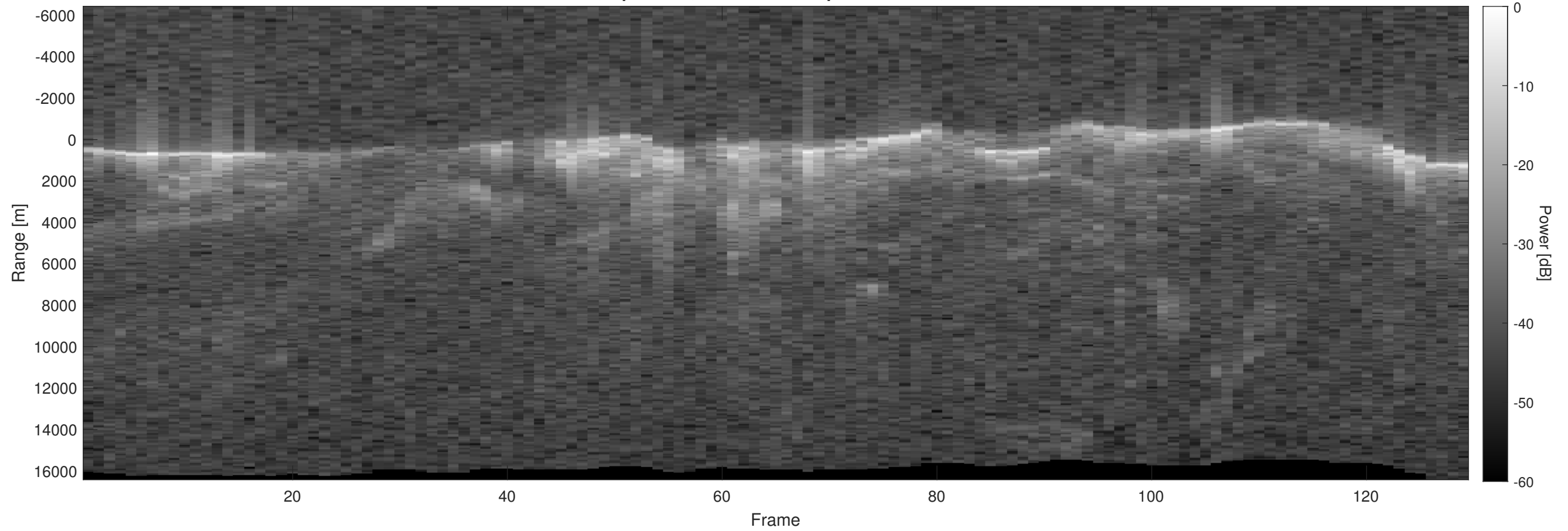
Orbit 4931, Optimized, No Window, Depth-Corrected, Channel 2
