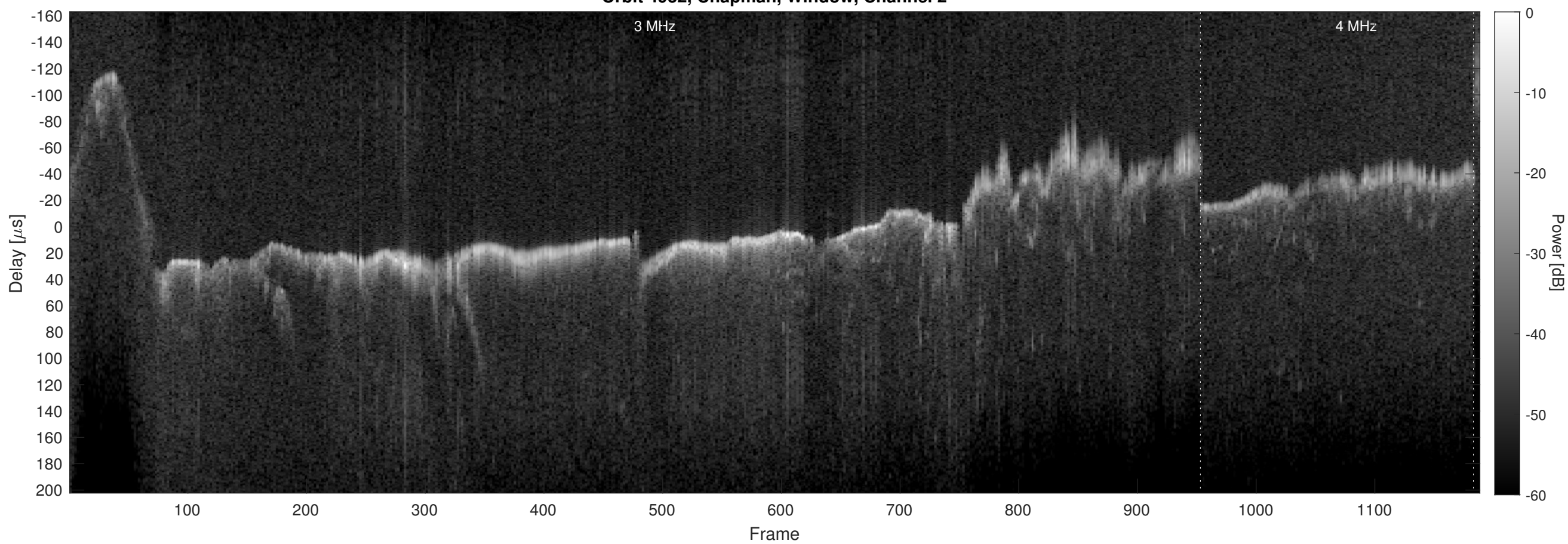
Orbit 4932, Chapman, Window, Channel 2
