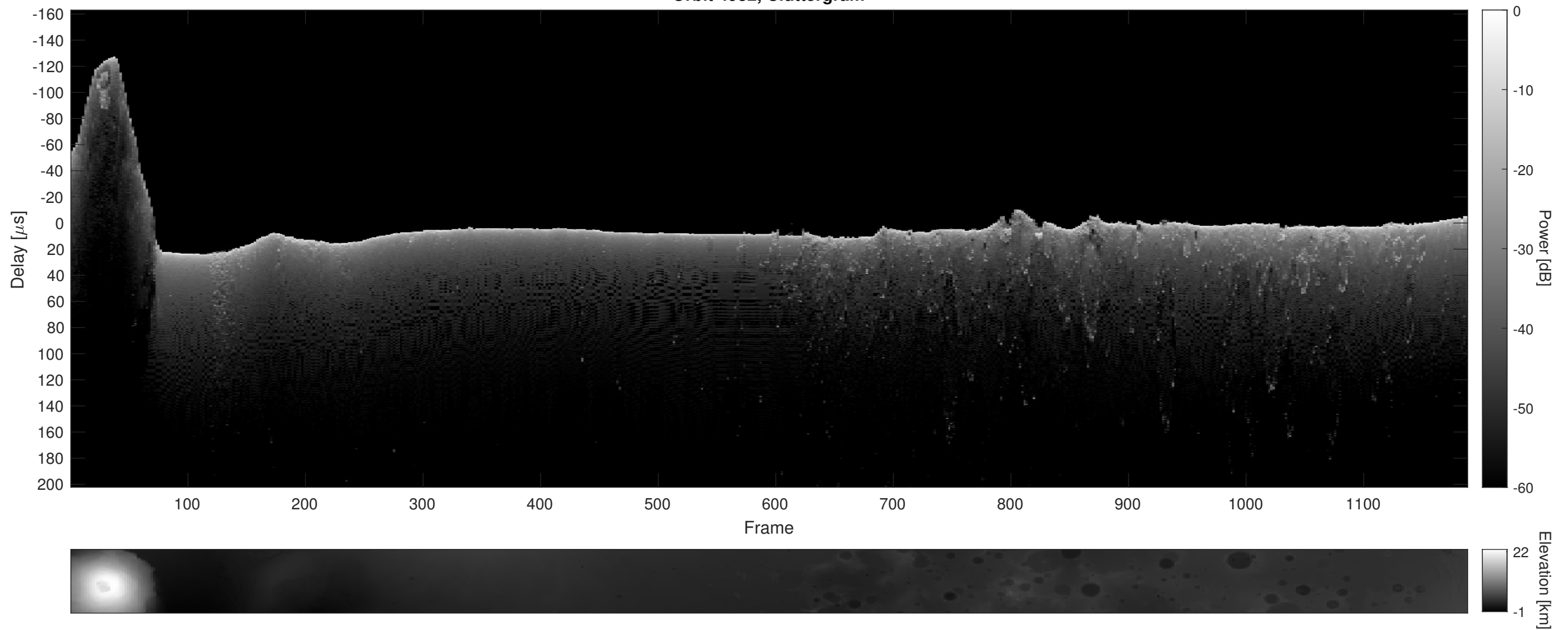
Orbit 4932, Cluttergram
