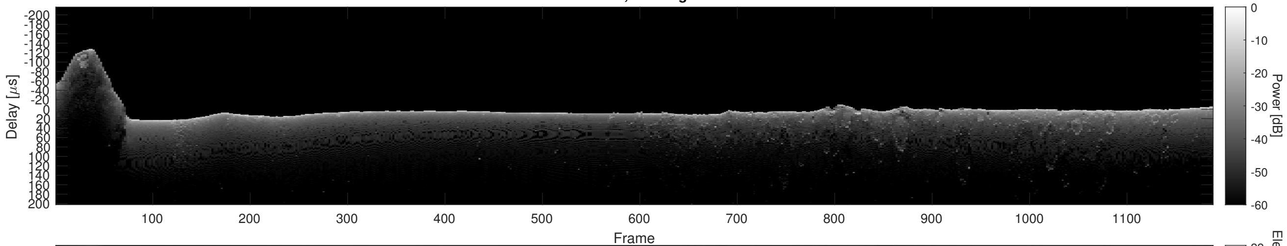
Orbit 4932, Cluttergram
