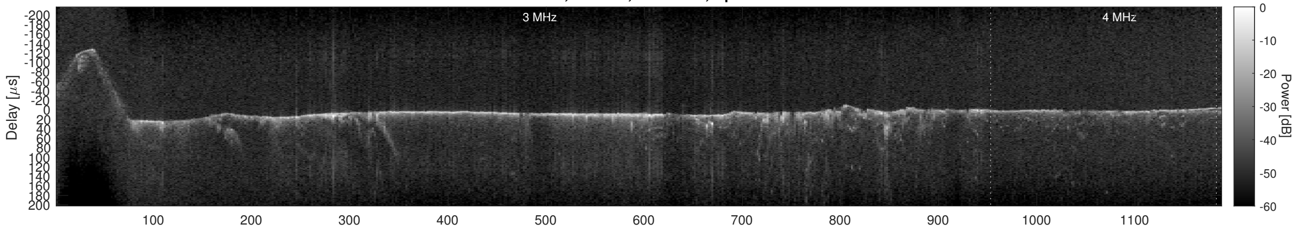
Orbit 4932, Cluttergram
