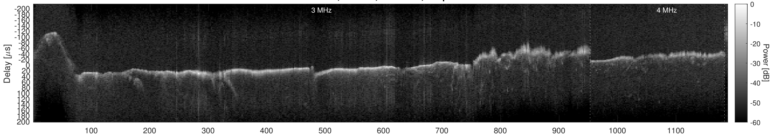
Orbit 4932, Window, Channel 2, Optimized
