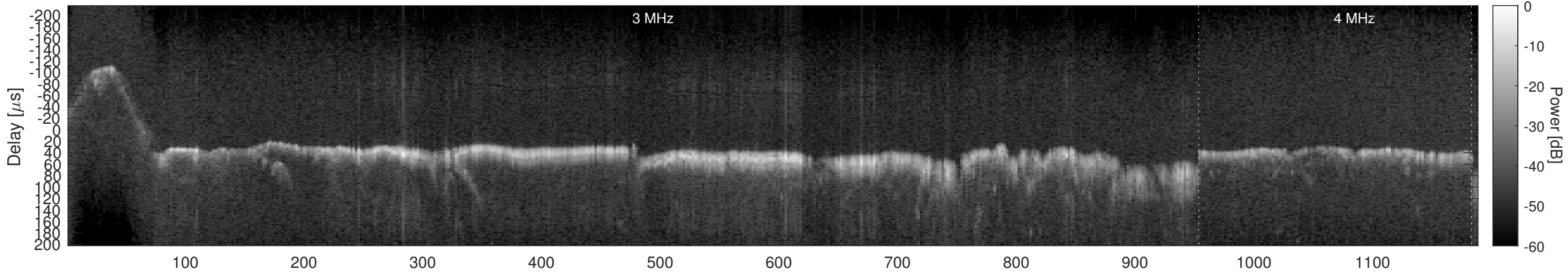
Orbit 4932, Window, Channel 2, Chapman
