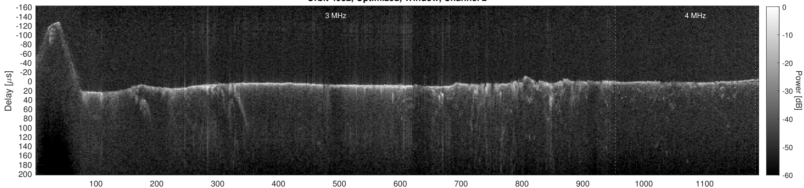
Orbit 4932, Cluttergram
