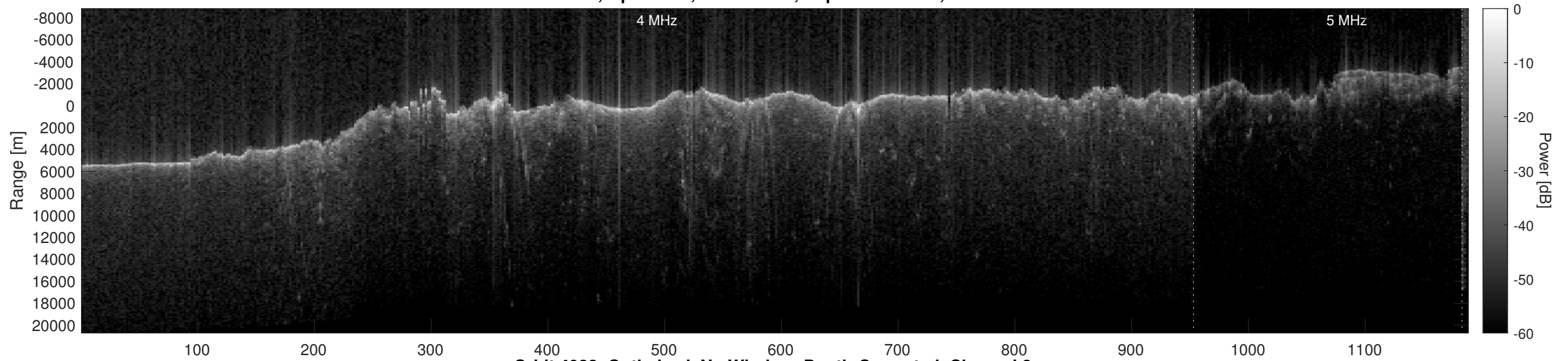
Orbit 4933, Optimized, No Window, Depth-Corrected, Channel 2
