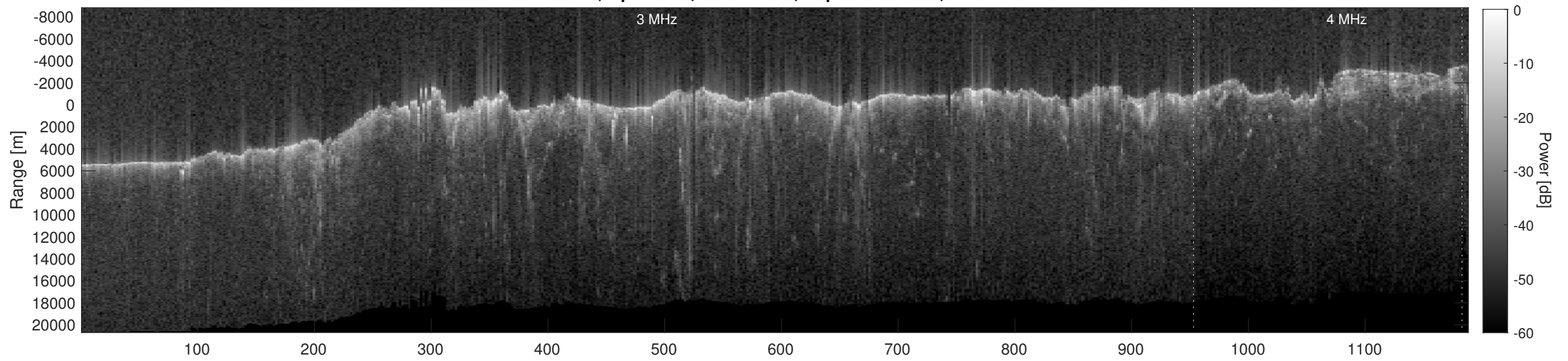
Orbit 4933, Depth-Corrected Cluttergram
