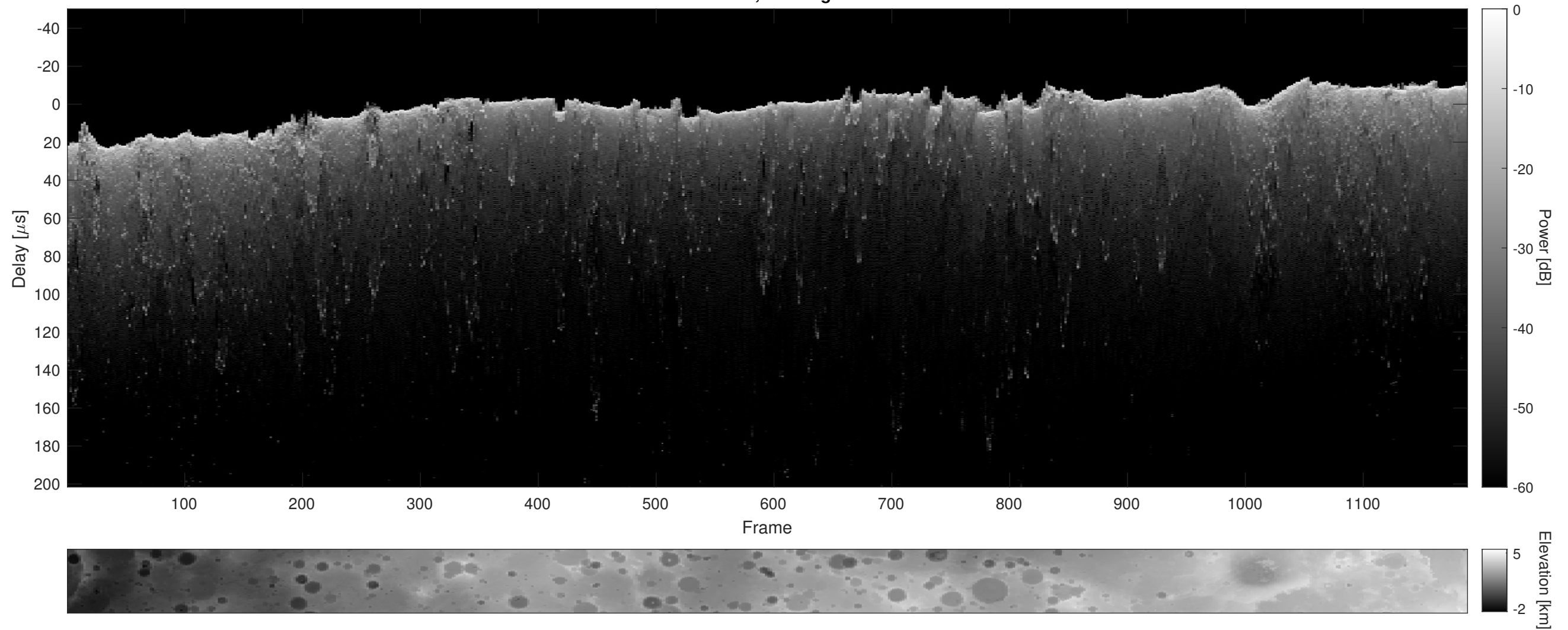
Orbit 4934, Cluttergram
