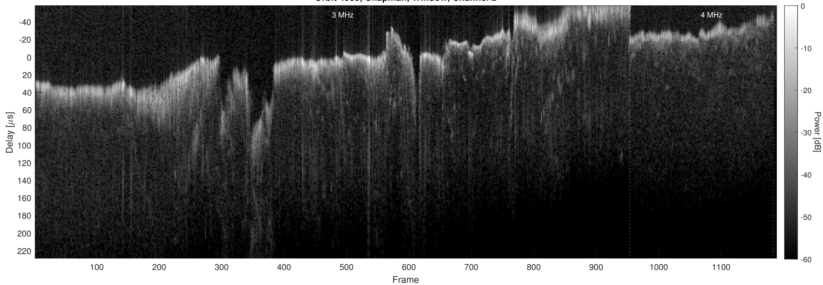
Orbit 4935, Chapman, Window, Channel 2
