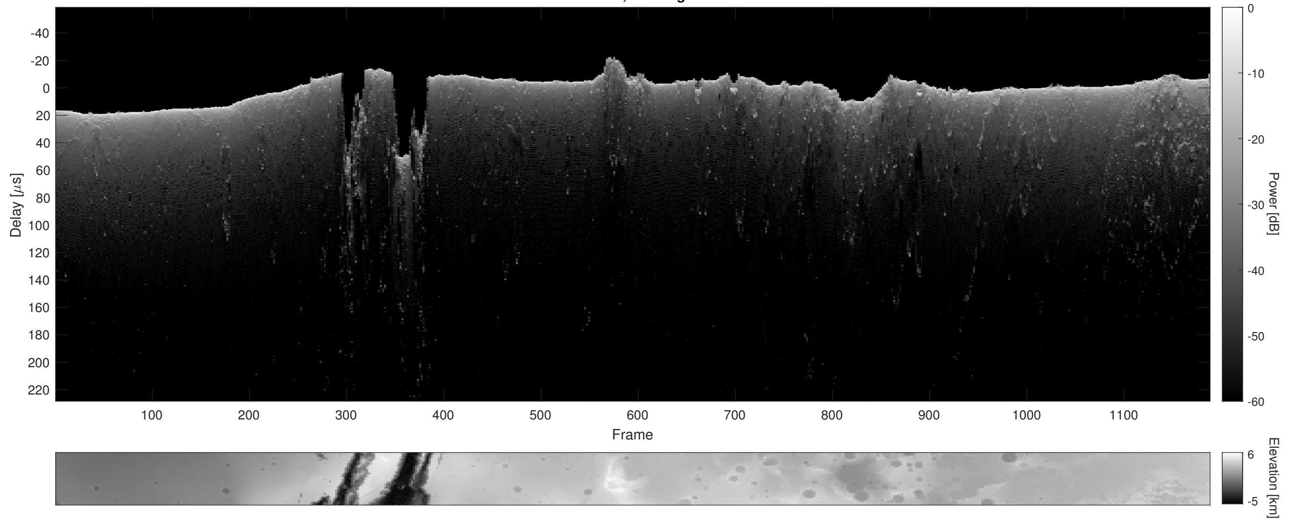
Orbit 4935, Cluttergram
