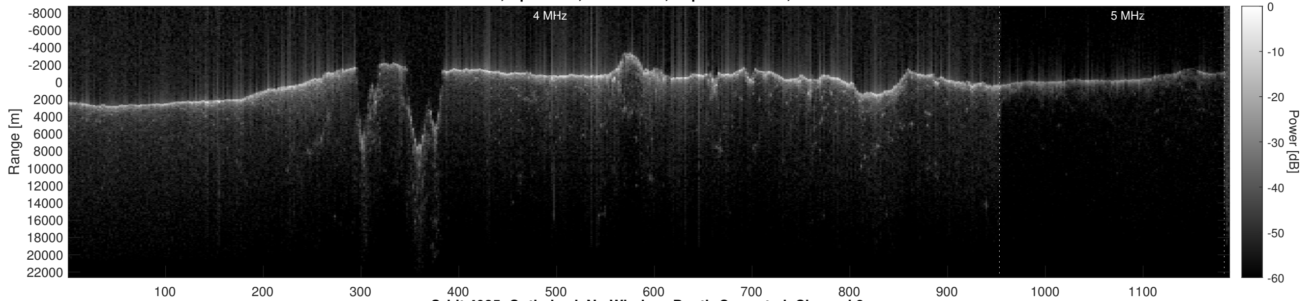
Orbit 4935, Optimized, No Window, Depth-Corrected, Channel 2
