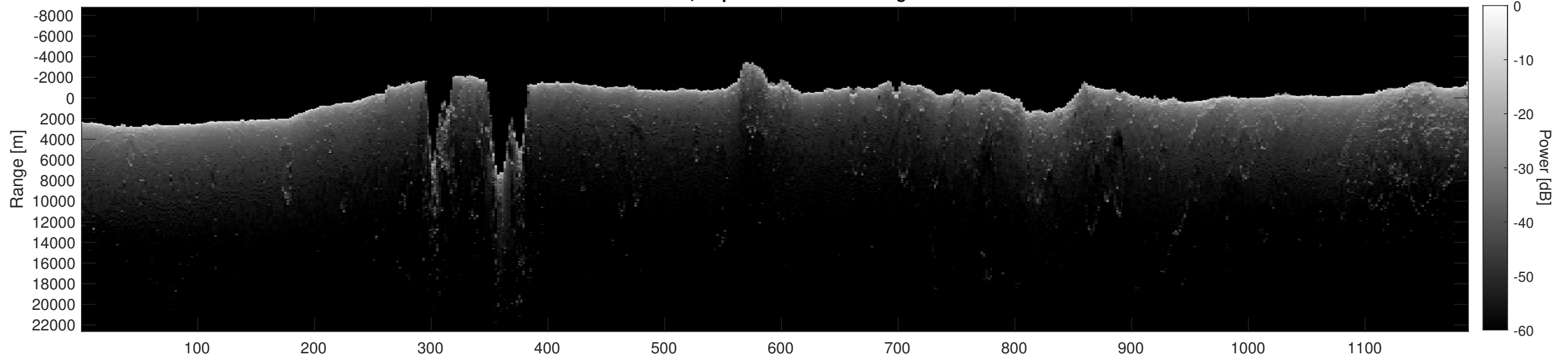
Orbit 4935, Depth-Corrected Cluttergram
