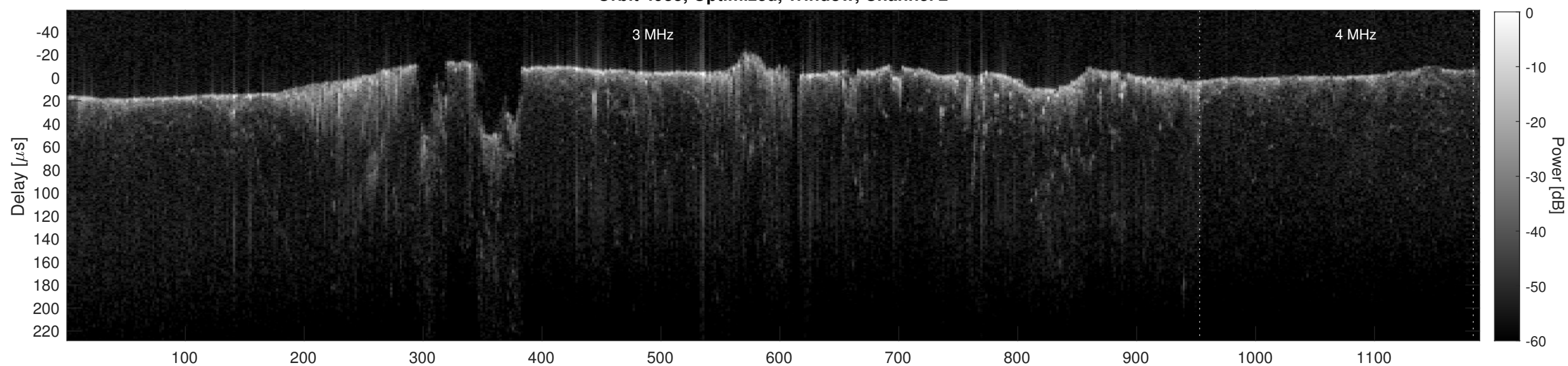
Orbit 4935, Cluttergram
