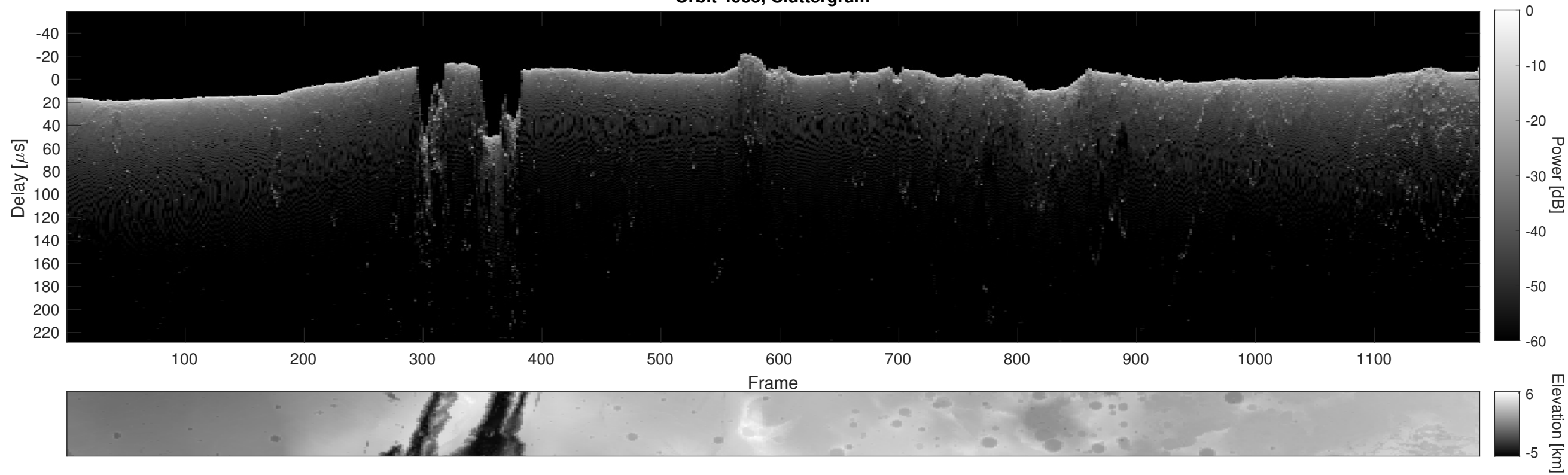
Orbit 4935, Cluttergram
