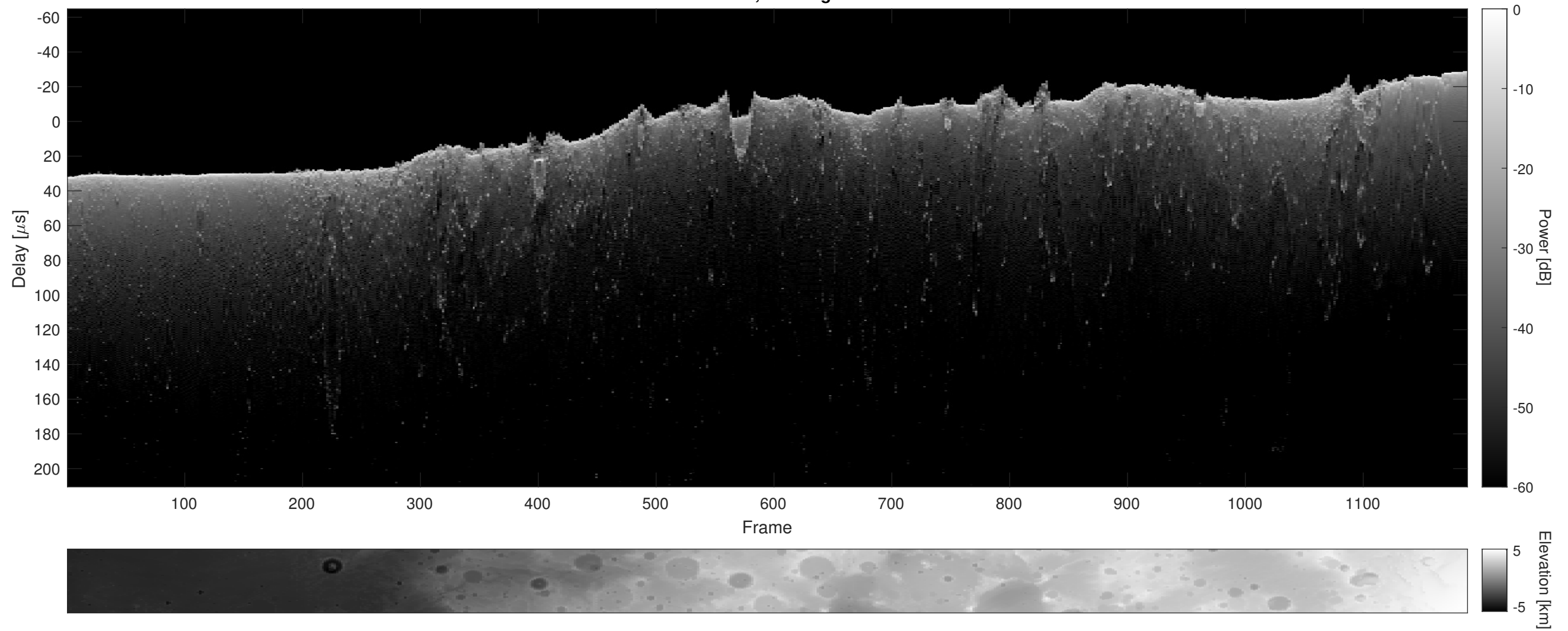
Orbit 4936, Cluttergram
