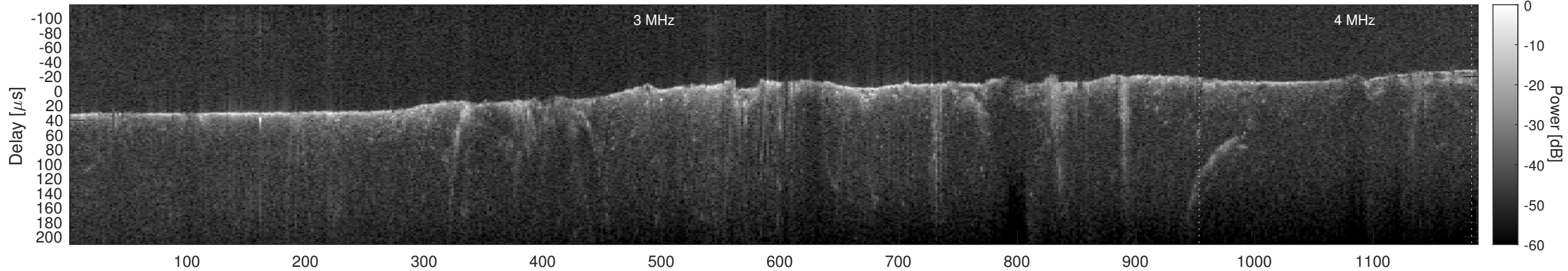
Orbit 4936, Cluttergram
