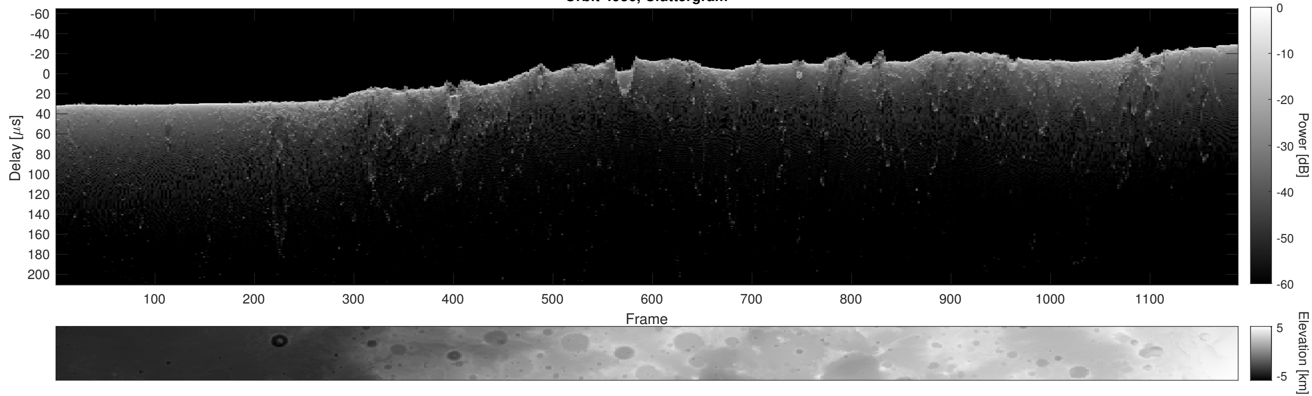
Orbit 4936, Cluttergram
