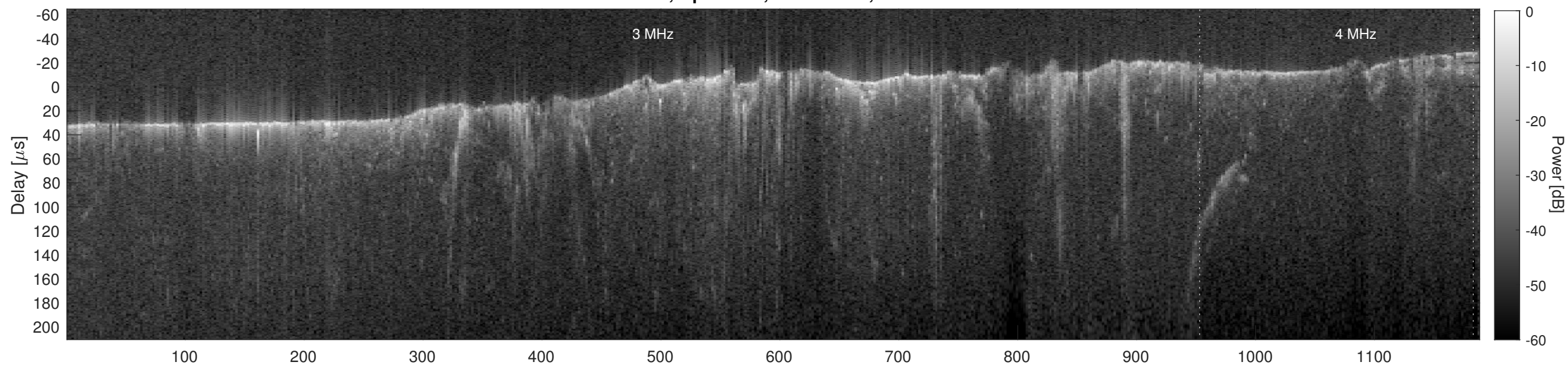
Orbit 4936, Cluttergram
