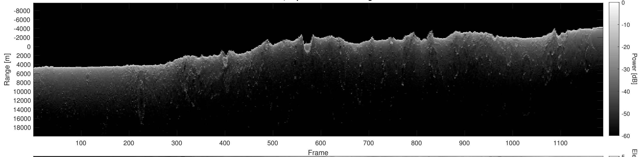
Orbit 4936, Depth-Corrected Cluttergram
