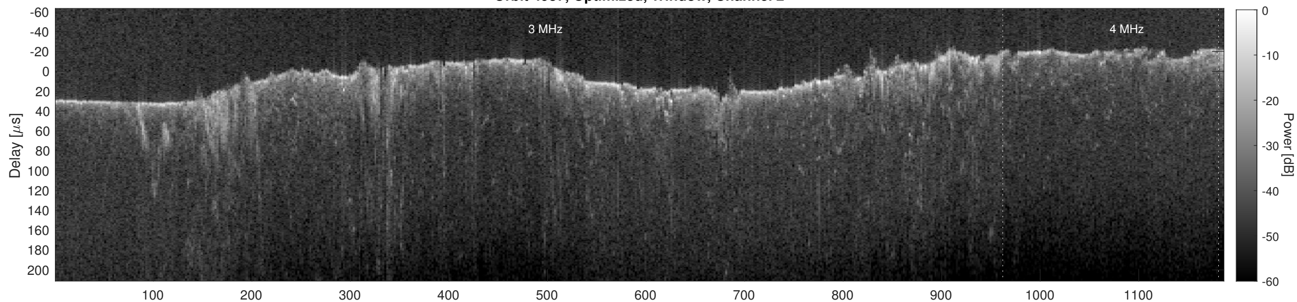
Orbit 4937, Cluttergram
