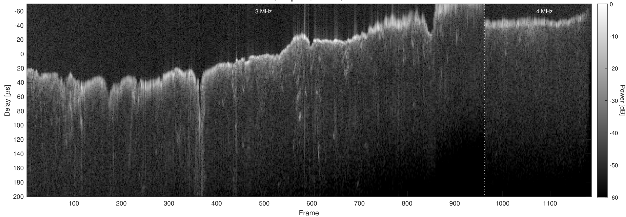
Orbit 4938, Chapman, Window, Channel 2
