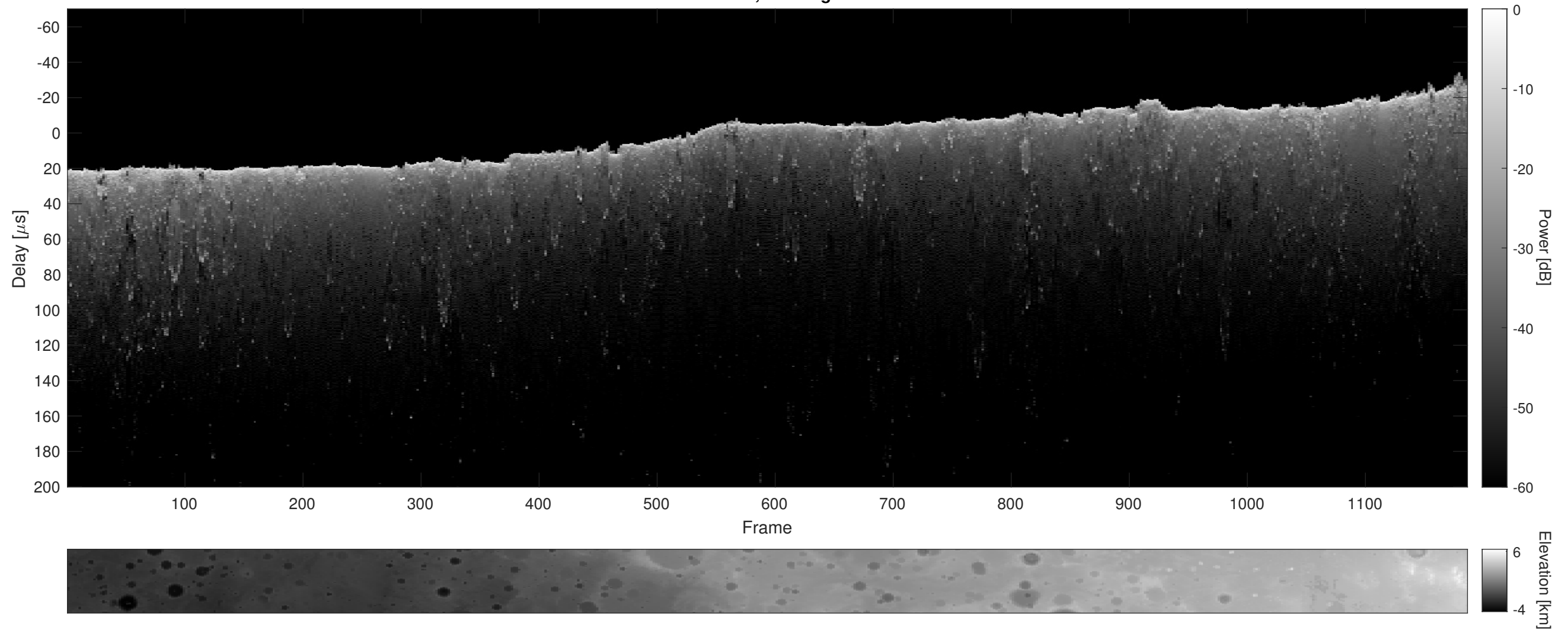
Orbit 4938, Cluttergram
