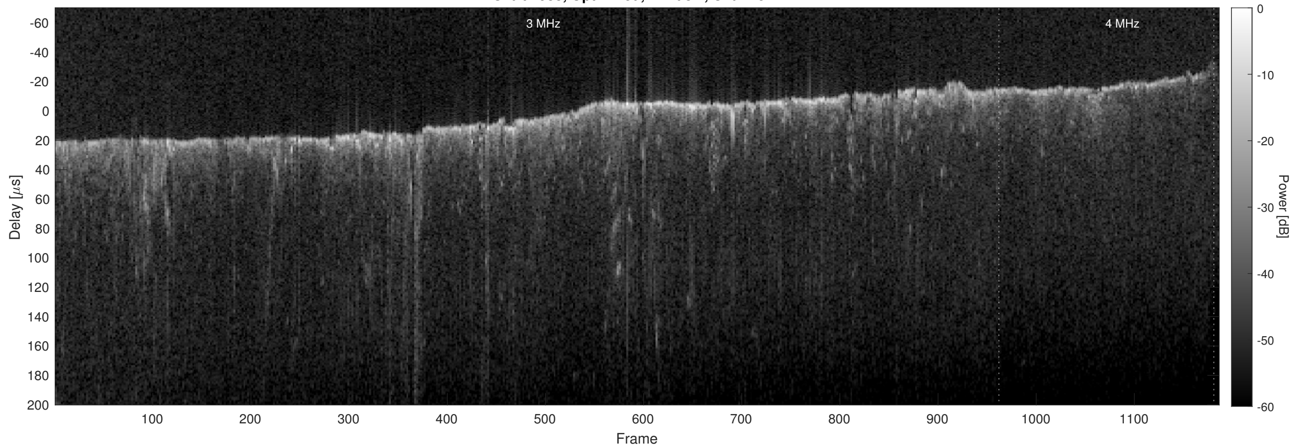
Orbit 4938, Optimized, Window, Channel 2
