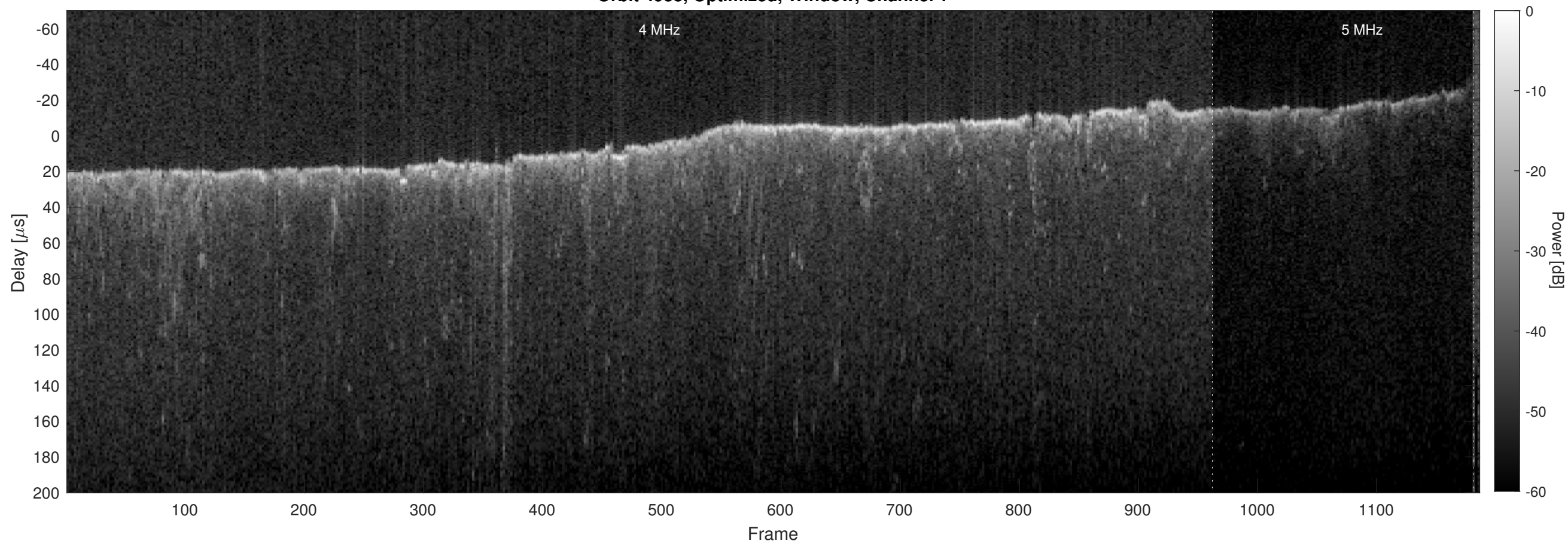
Orbit 4938, Optimized, Window, Channel 2
