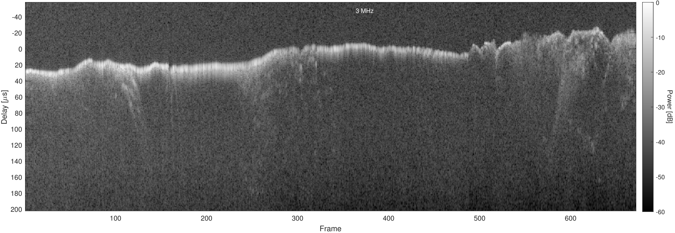
Orbit 4939, Chapman, Window, Channel 2
