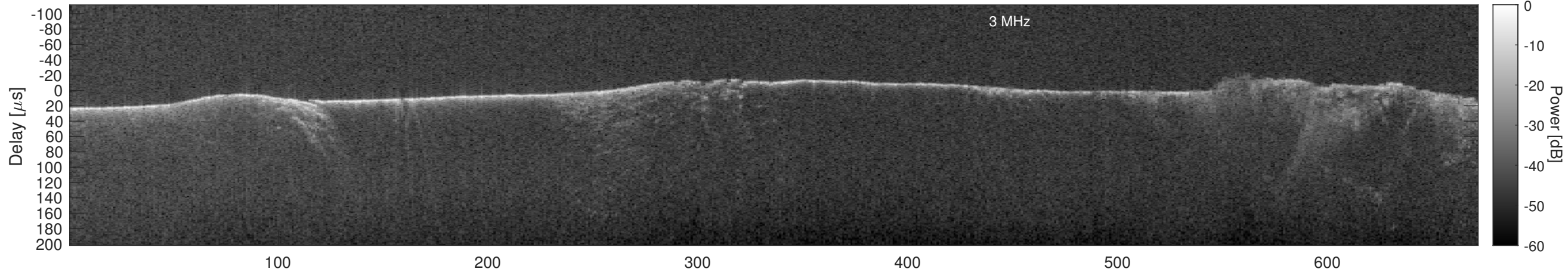
Orbit 4939, Cluttergram
