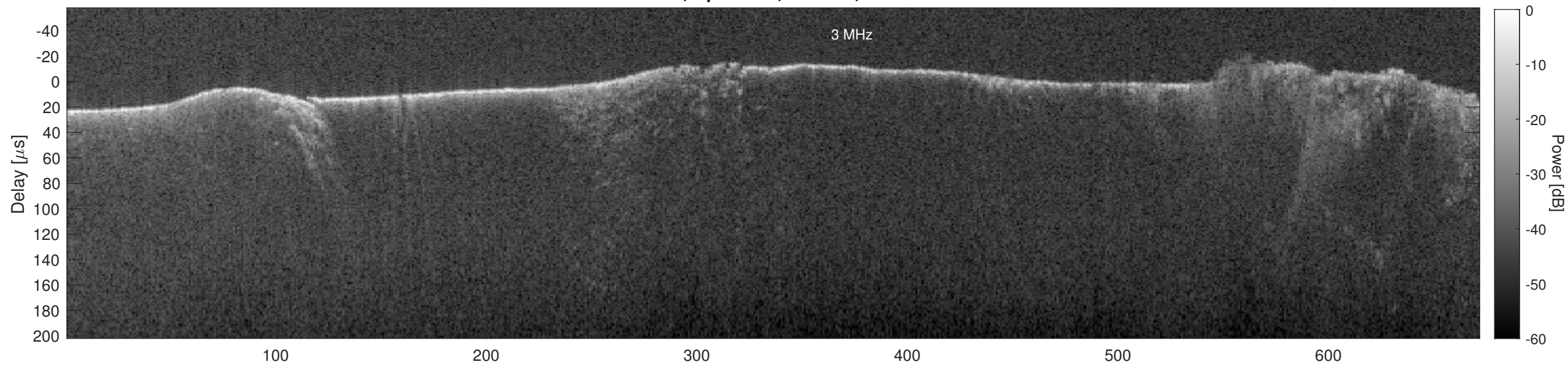
Orbit 4939, Cluttergram
