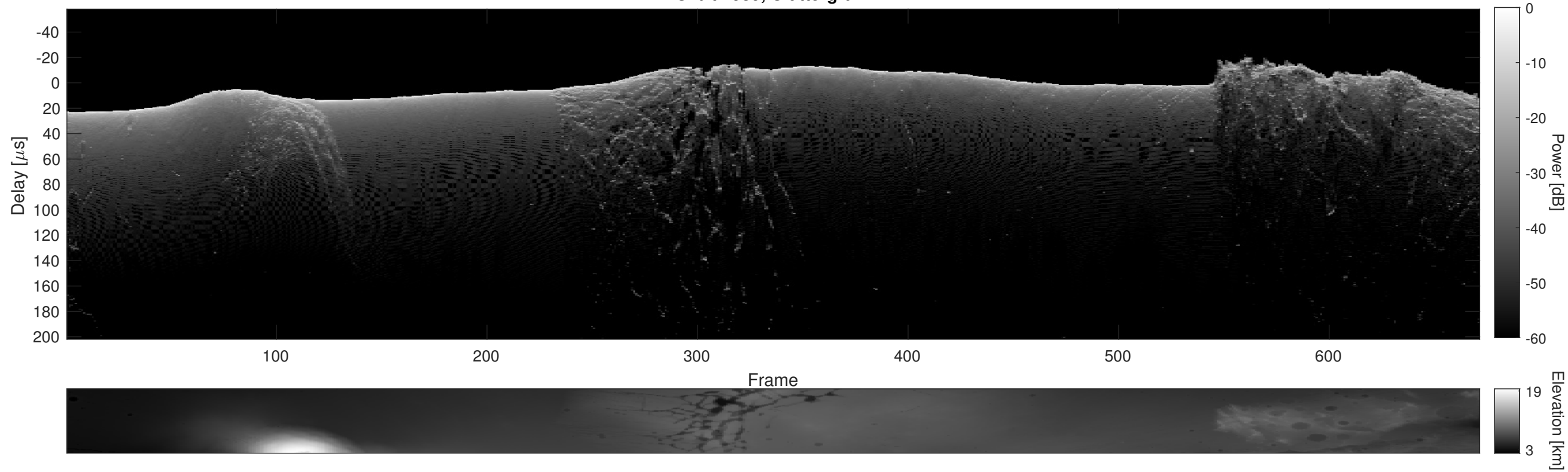
Orbit 4939, Cluttergram
