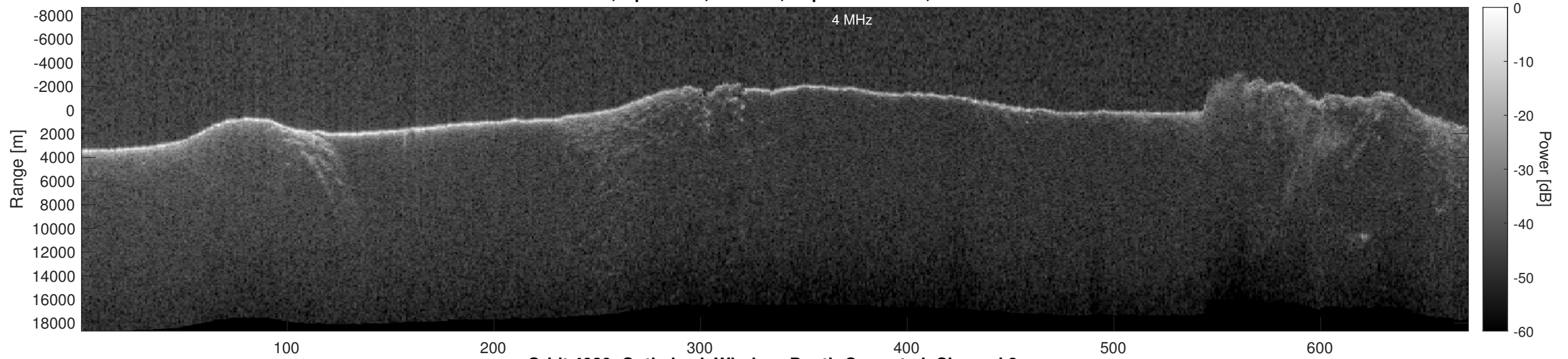
Orbit 4939, Optimized, Window, Depth-Corrected, Channel 2
