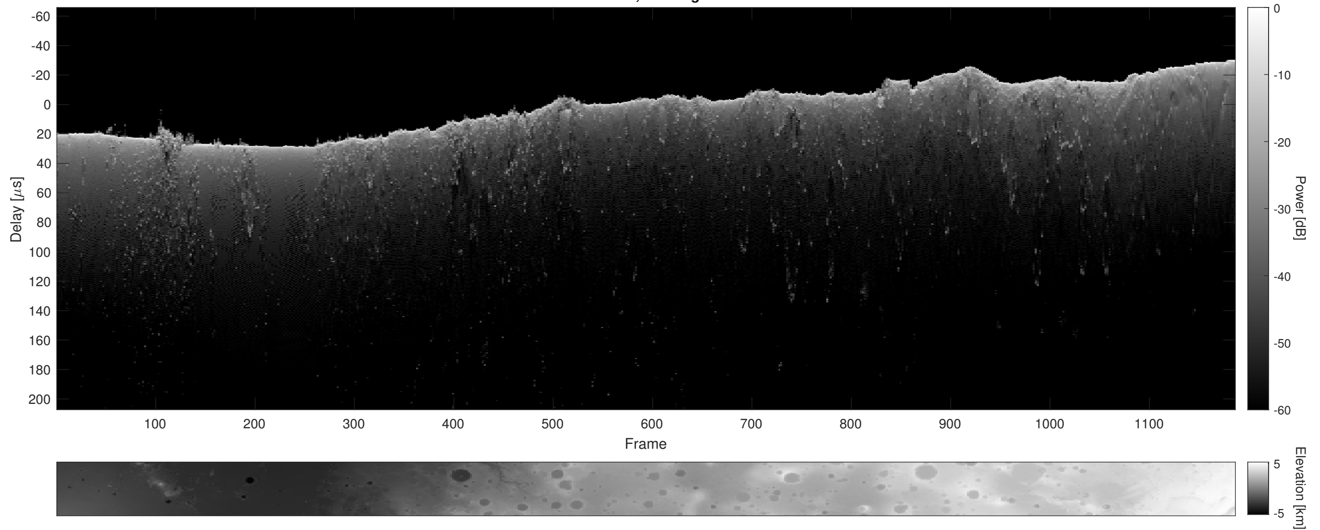
Orbit 4940, Cluttergram
