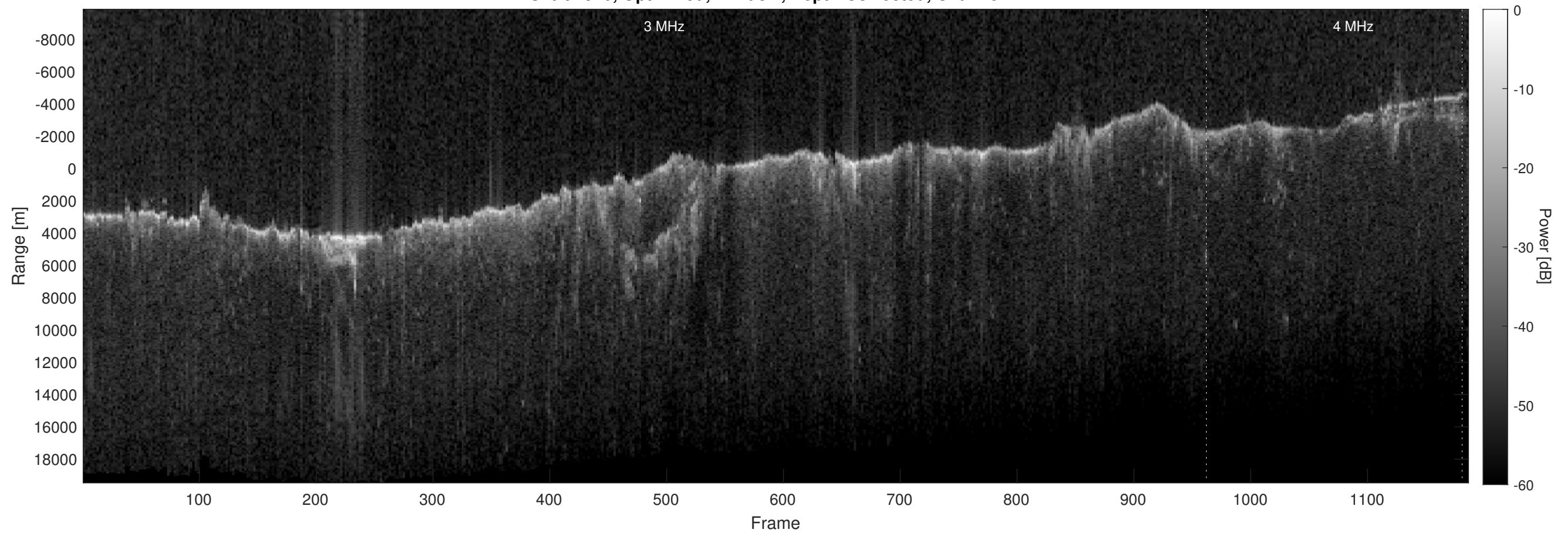
Orbit 4940, Optimized, Window, Depth-Corrected, Channel 2
