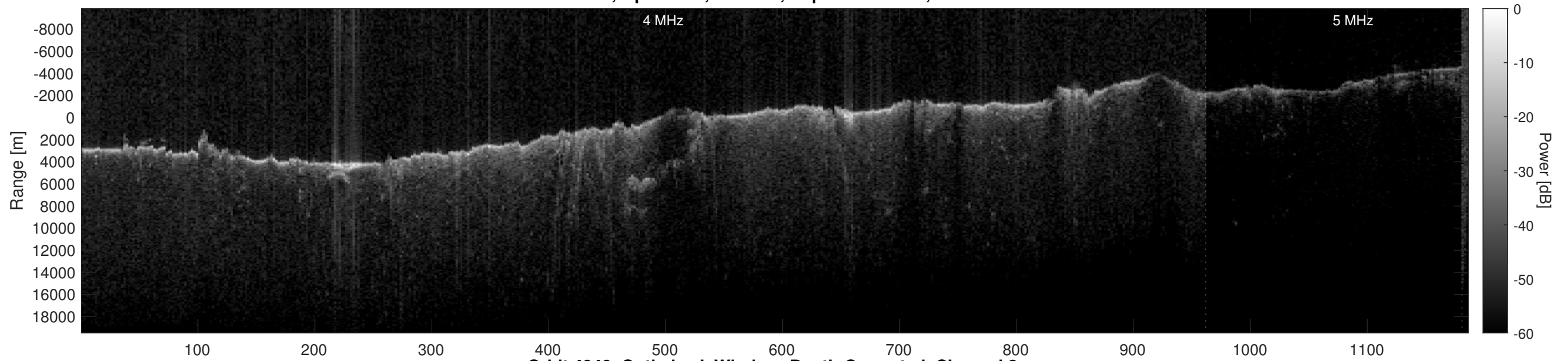
Orbit 4940, Optimized, Window, Depth-Corrected, Channel 2
