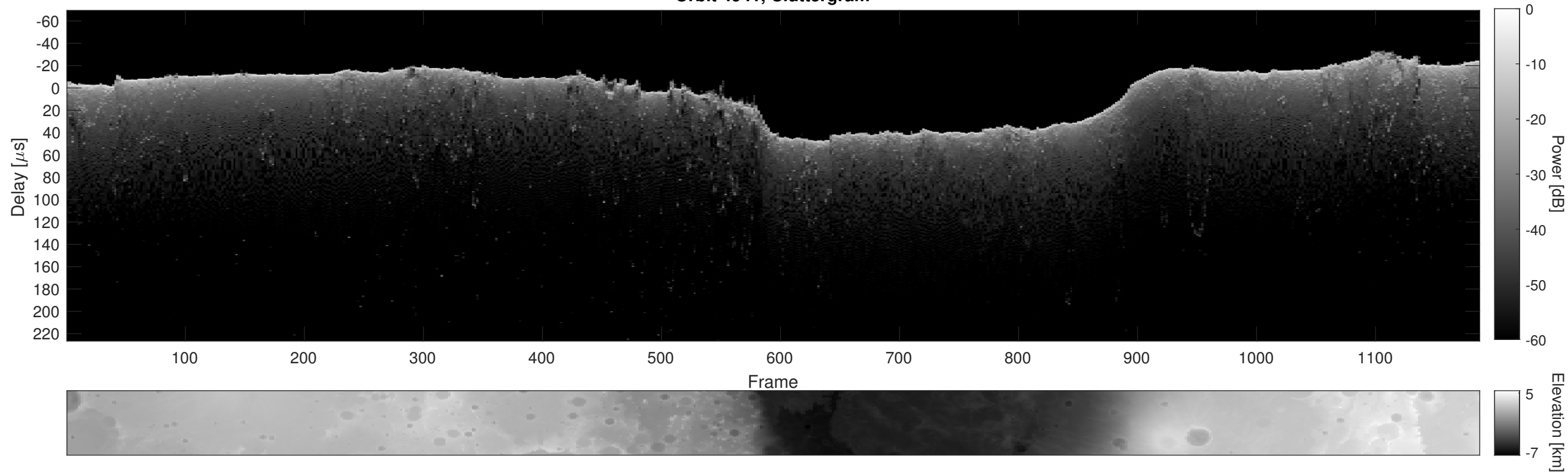
Orbit 4941, Cluttergram
