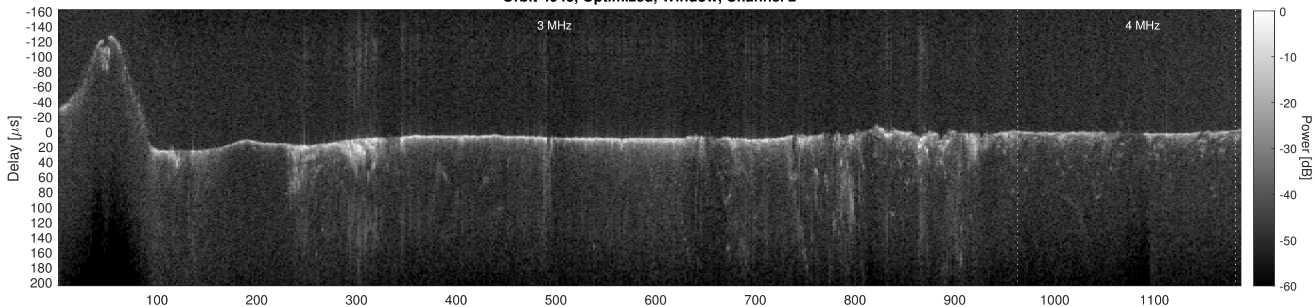
Orbit 4943, Cluttergram
