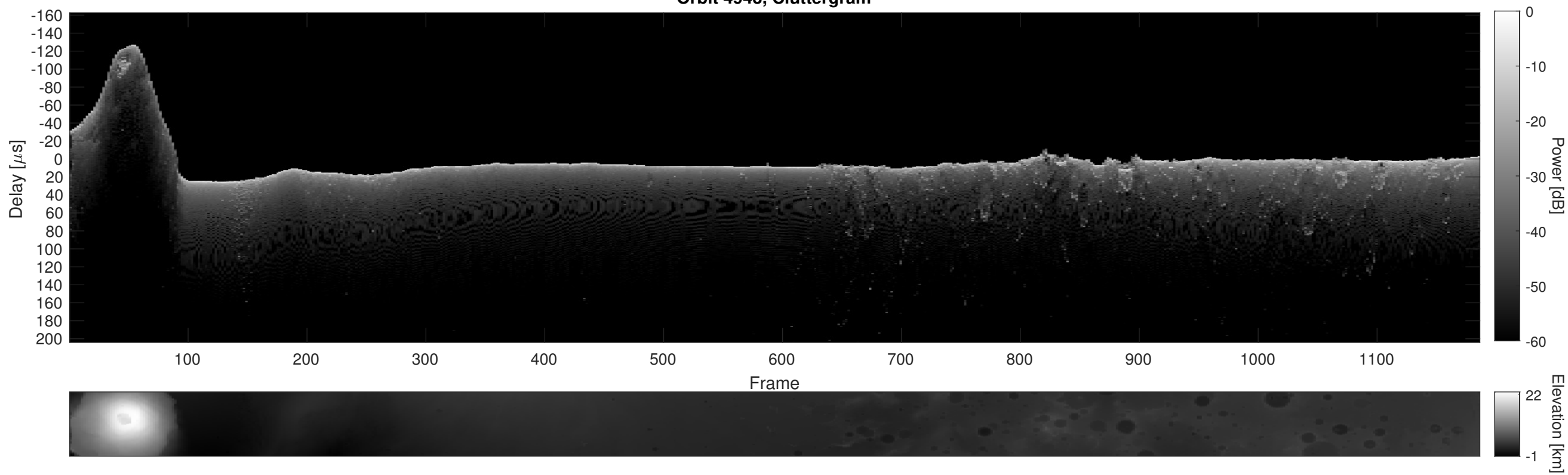
Orbit 4943, Cluttergram
