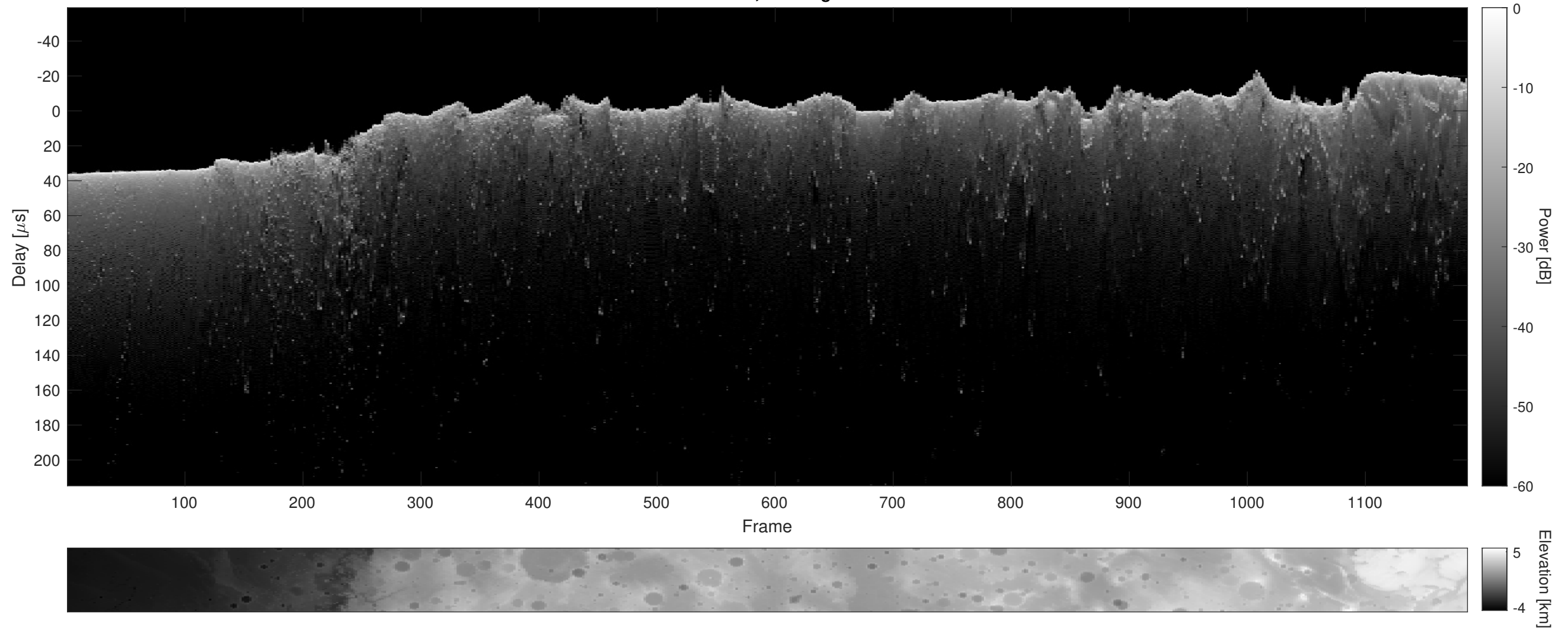
Orbit 4944, Cluttergram
