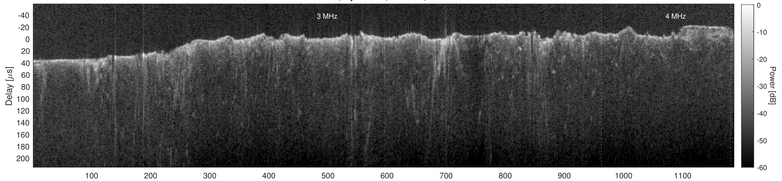
Orbit 4944, Cluttergram
