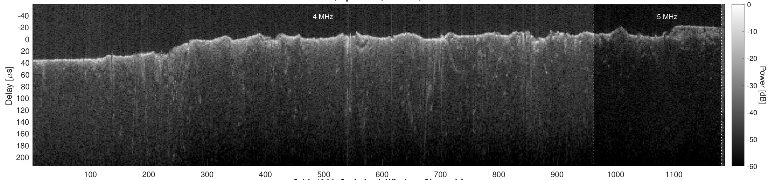
Orbit 4944, Optimized, Window, Channel 2
