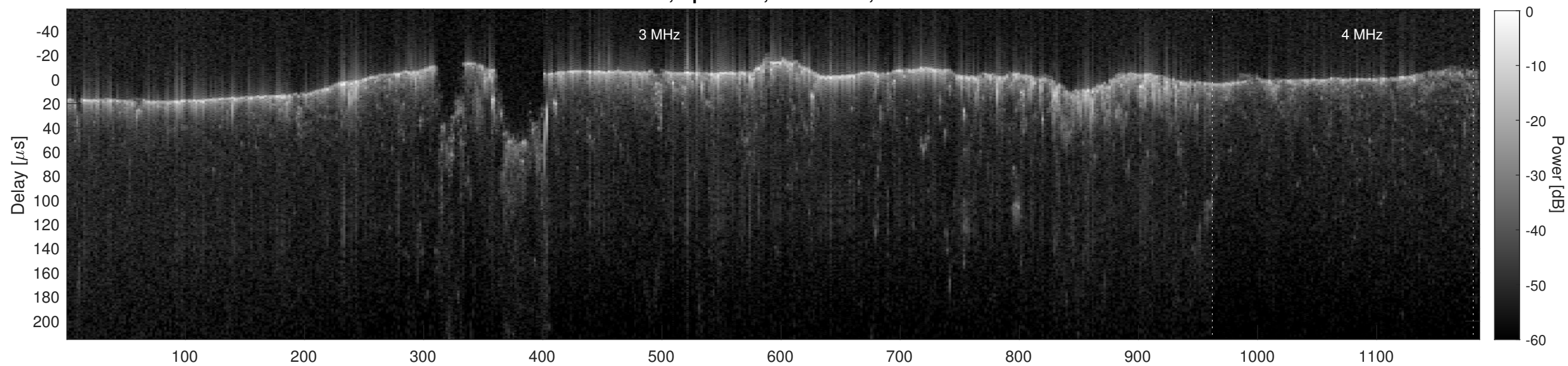
Orbit 4946, Cluttergram
