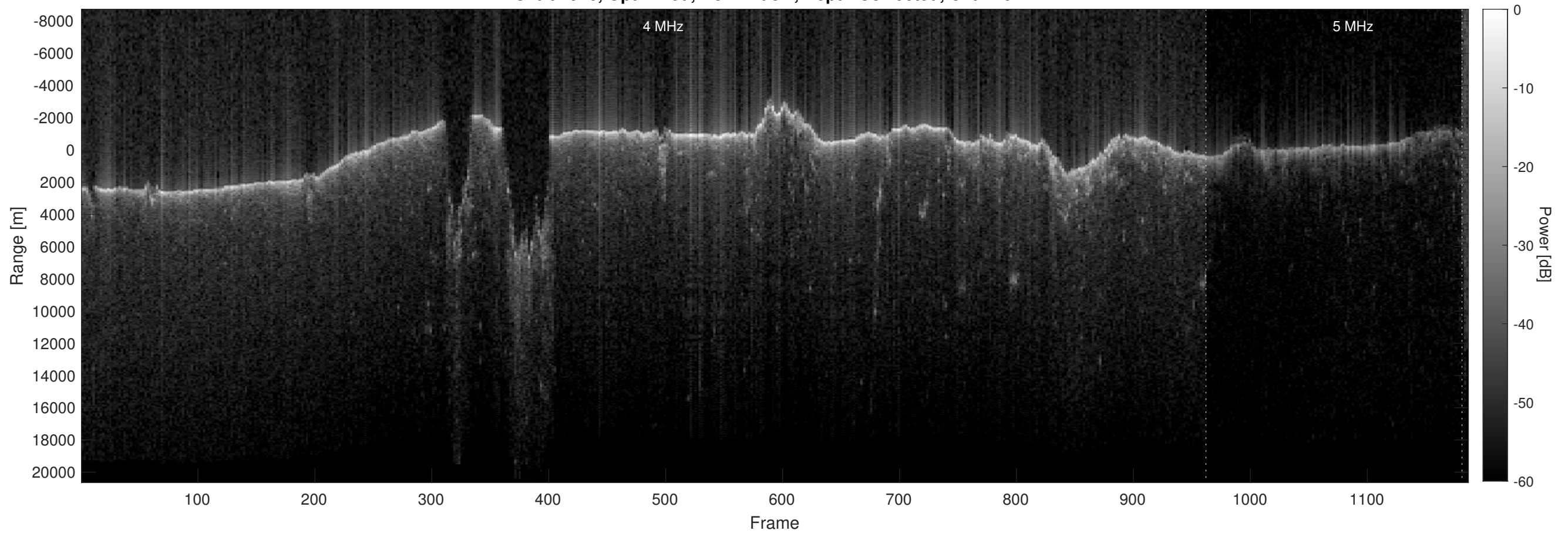
Orbit 4946, Optimized, No Window, Depth-Corrected, Channel 2
