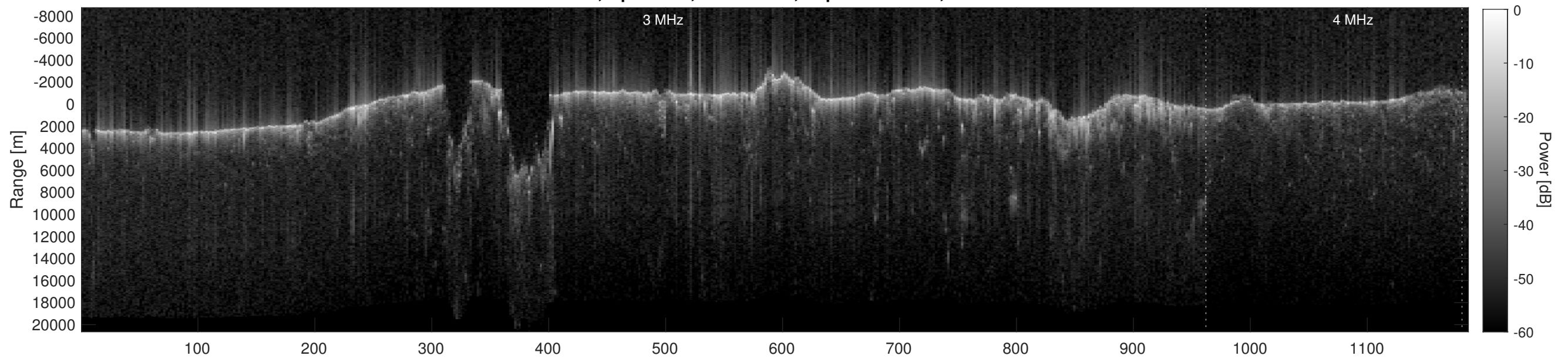
Orbit 4946, Depth-Corrected Cluttergram
