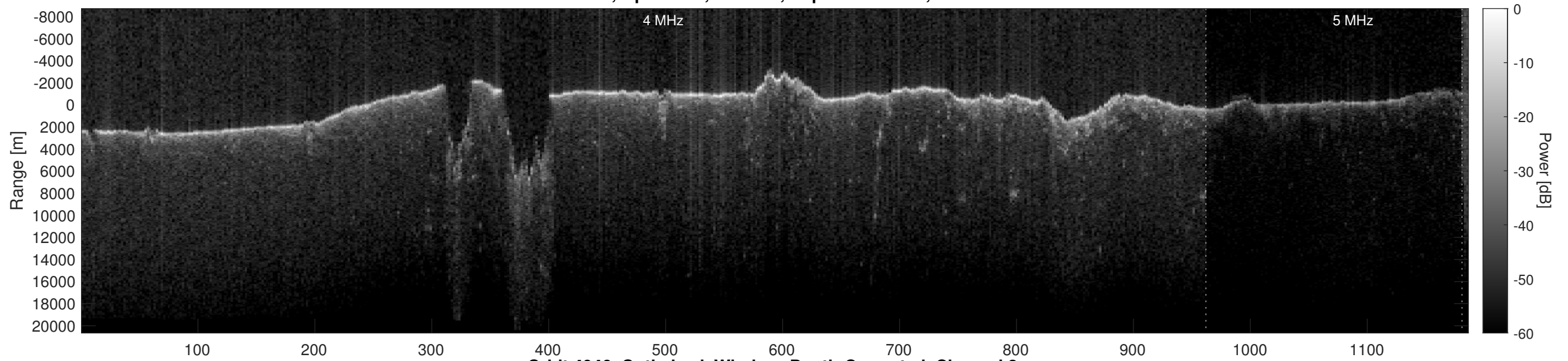
Orbit 4946, Optimized, Window, Depth-Corrected, Channel 2
