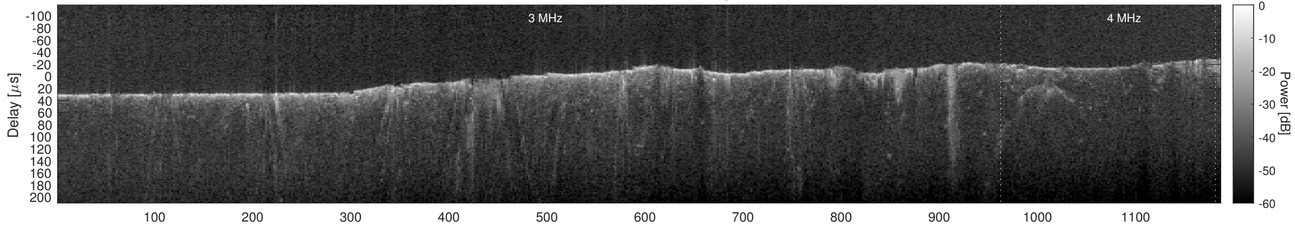
Orbit 4947, Cluttergram
