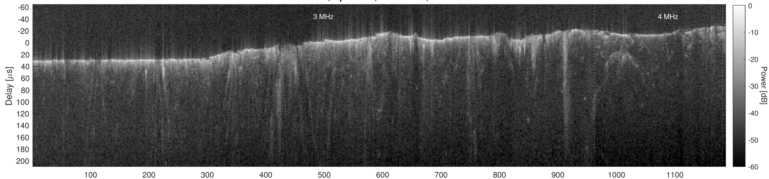
Orbit 4947, Cluttergram
