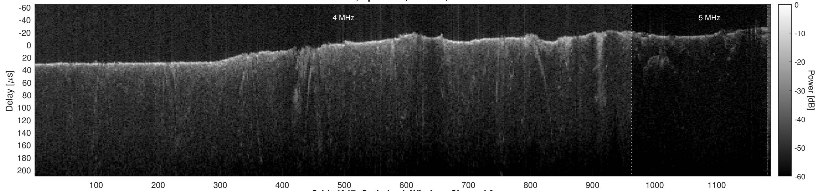
Orbit 4947, Optimized, Window, Channel 2
