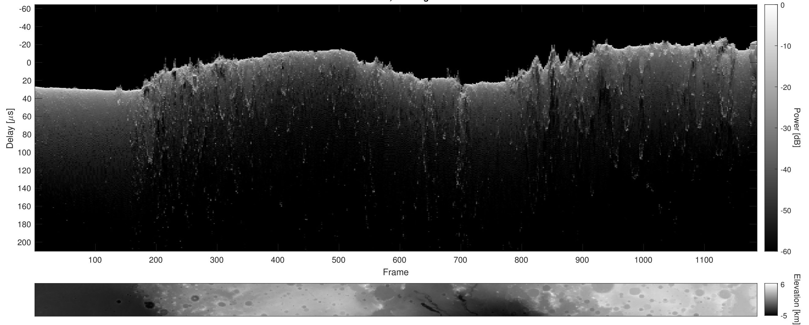
Orbit 4948, Cluttergram
