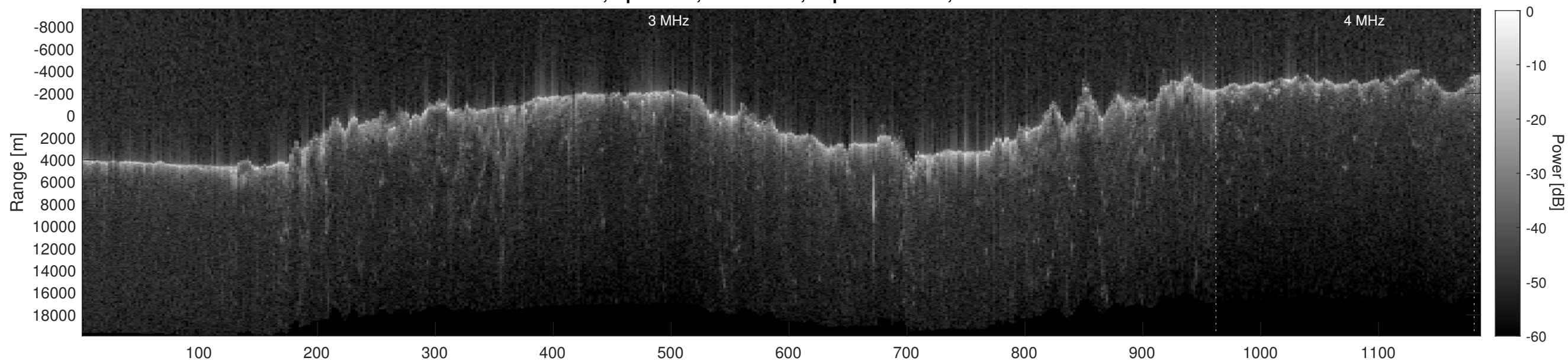
Orbit 4948, Depth-Corrected Cluttergram
