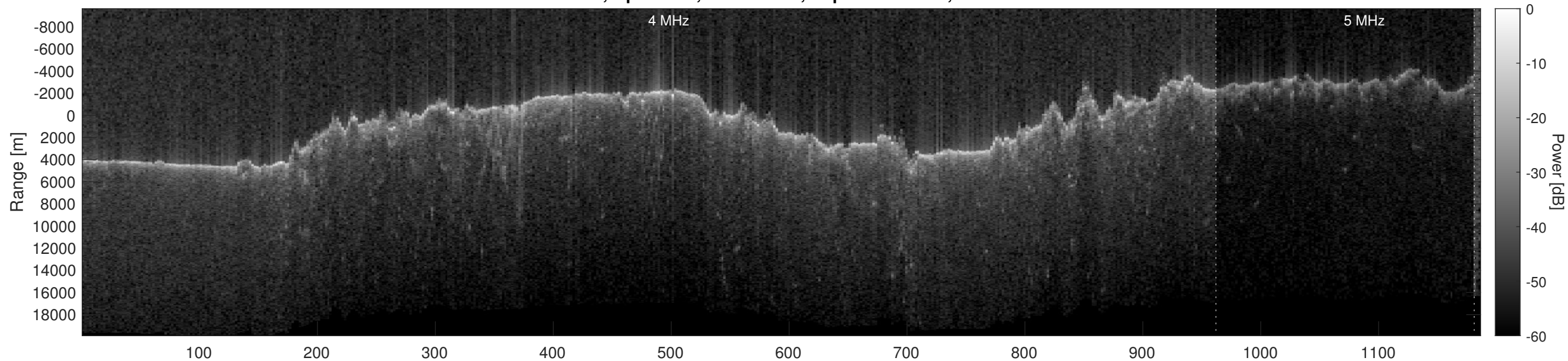
Orbit 4948, Optimized, No Window, Depth-Corrected, Channel 2
