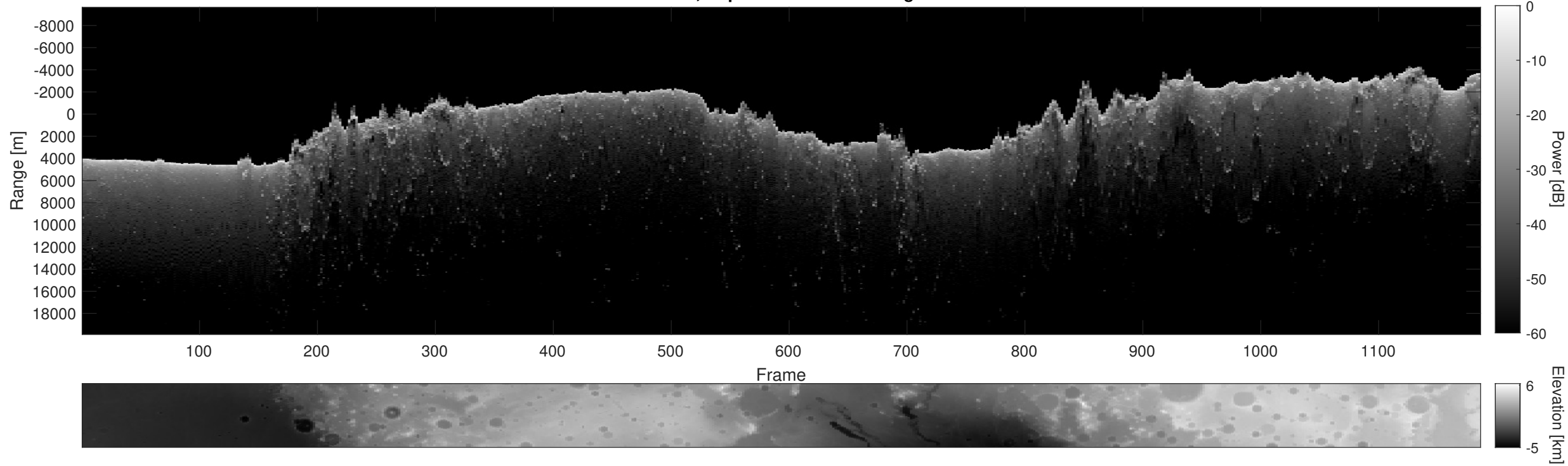
Orbit 4948, Depth-Corrected Cluttergram
