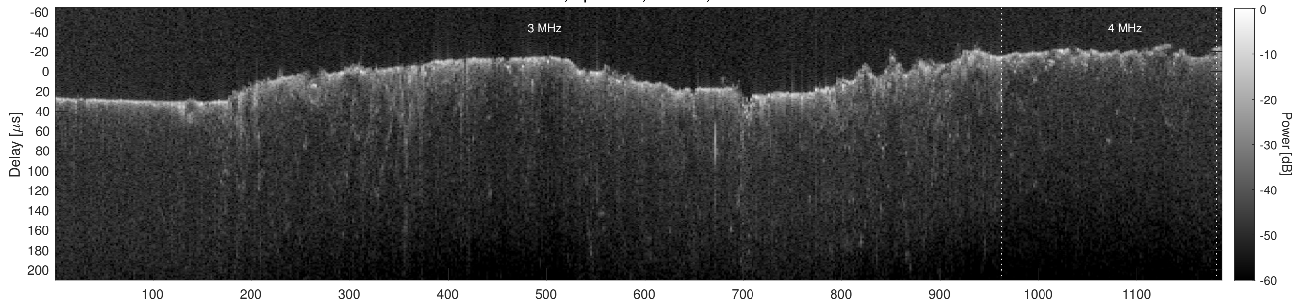
Orbit 4948, Cluttergram
