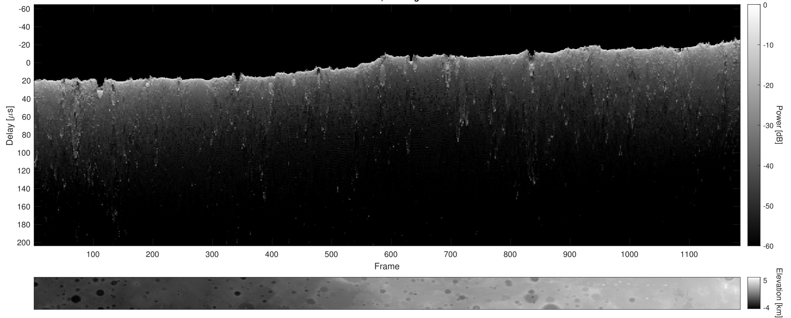
Orbit 4949, Cluttergram
