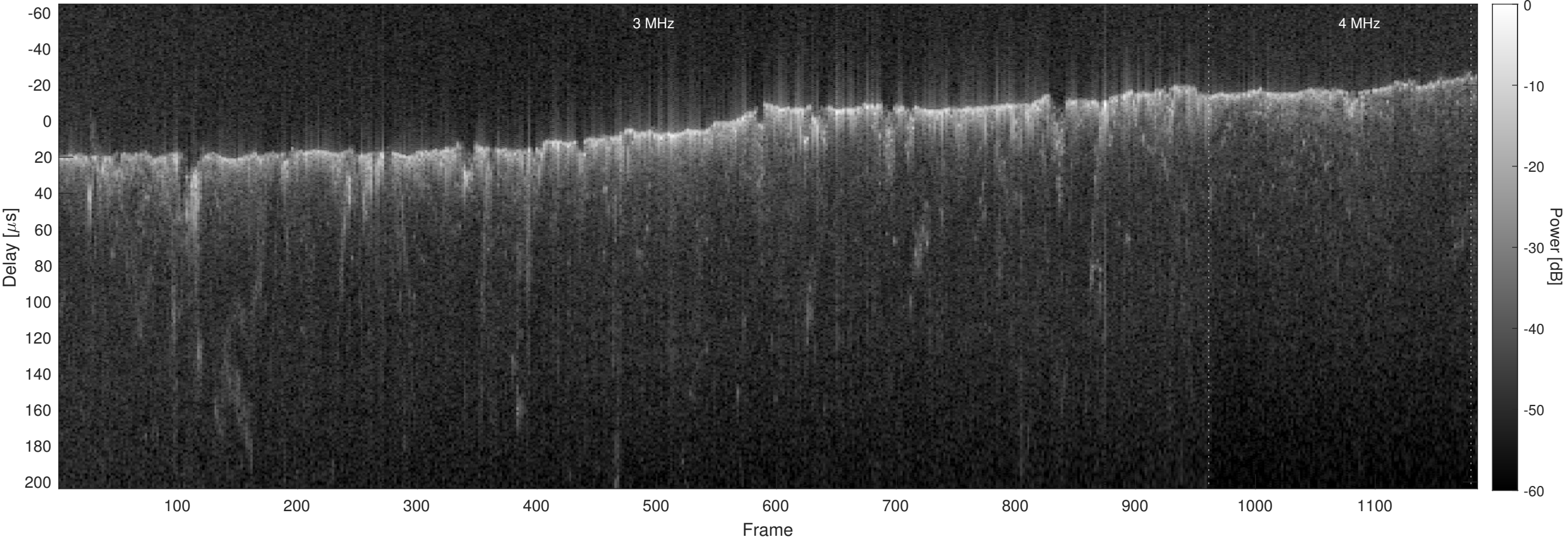
Orbit 4949, Optimized, No Window, Channel 2
