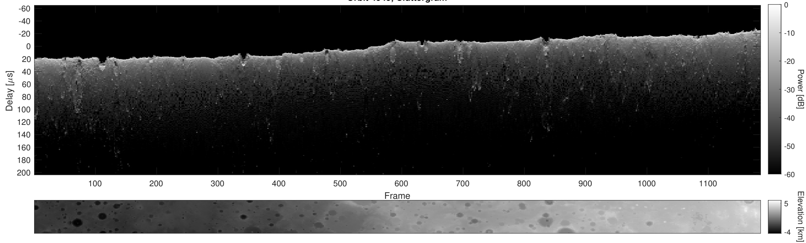
Orbit 4949, Cluttergram
