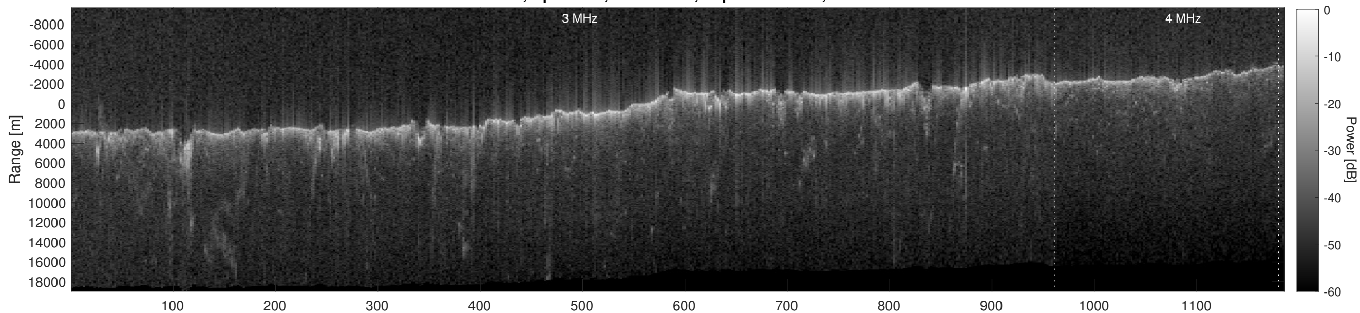
Orbit 4949, Depth-Corrected Cluttergram
