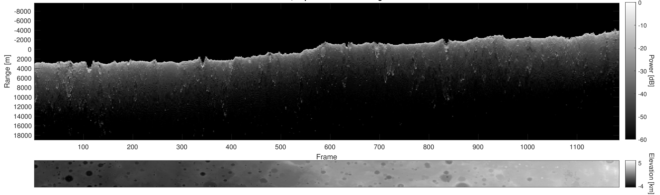
Orbit 4949, Depth-Corrected Cluttergram
