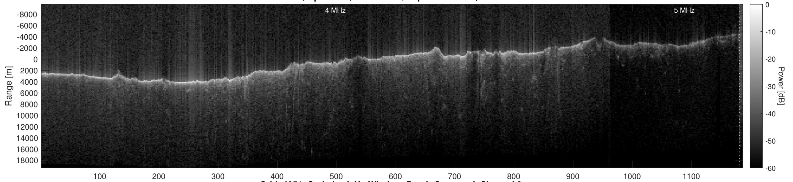
Orbit 4951, Optimized, No Window, Depth-Corrected, Channel 2
