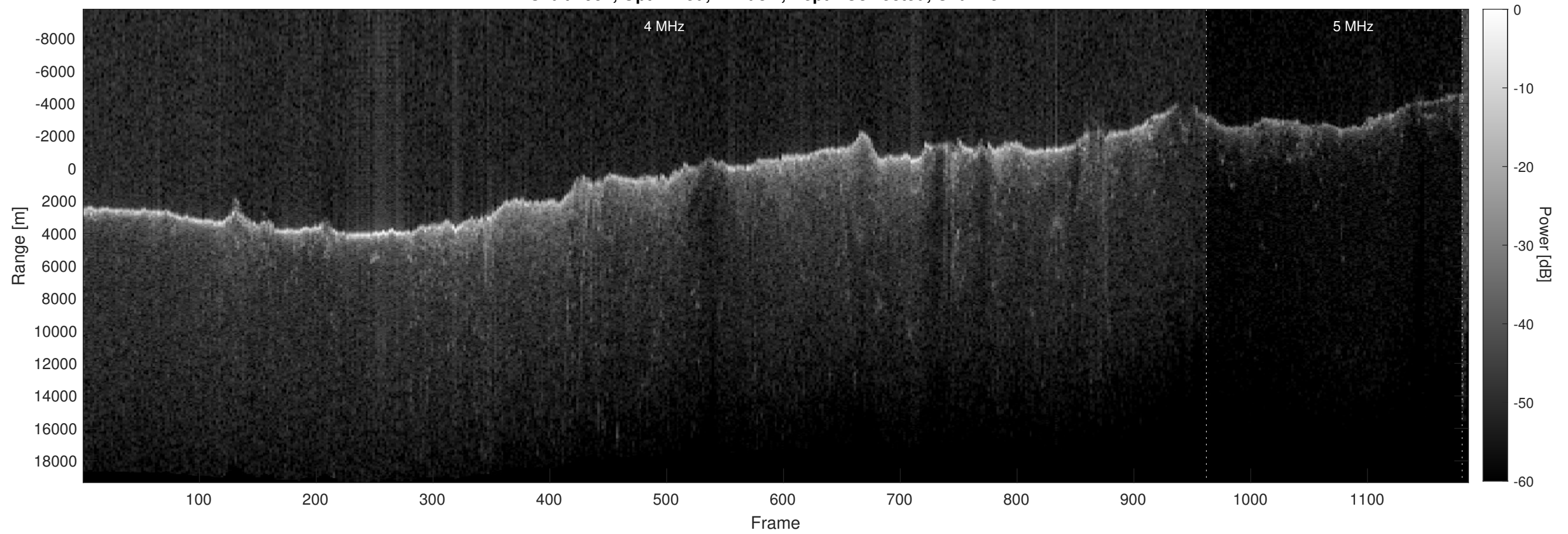
Orbit 4951, Optimized, Window, Depth-Corrected, Channel 2
