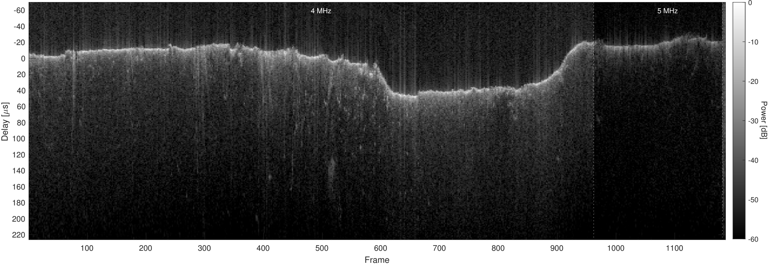
Orbit 4952, Optimized, No Window, Channel 2
